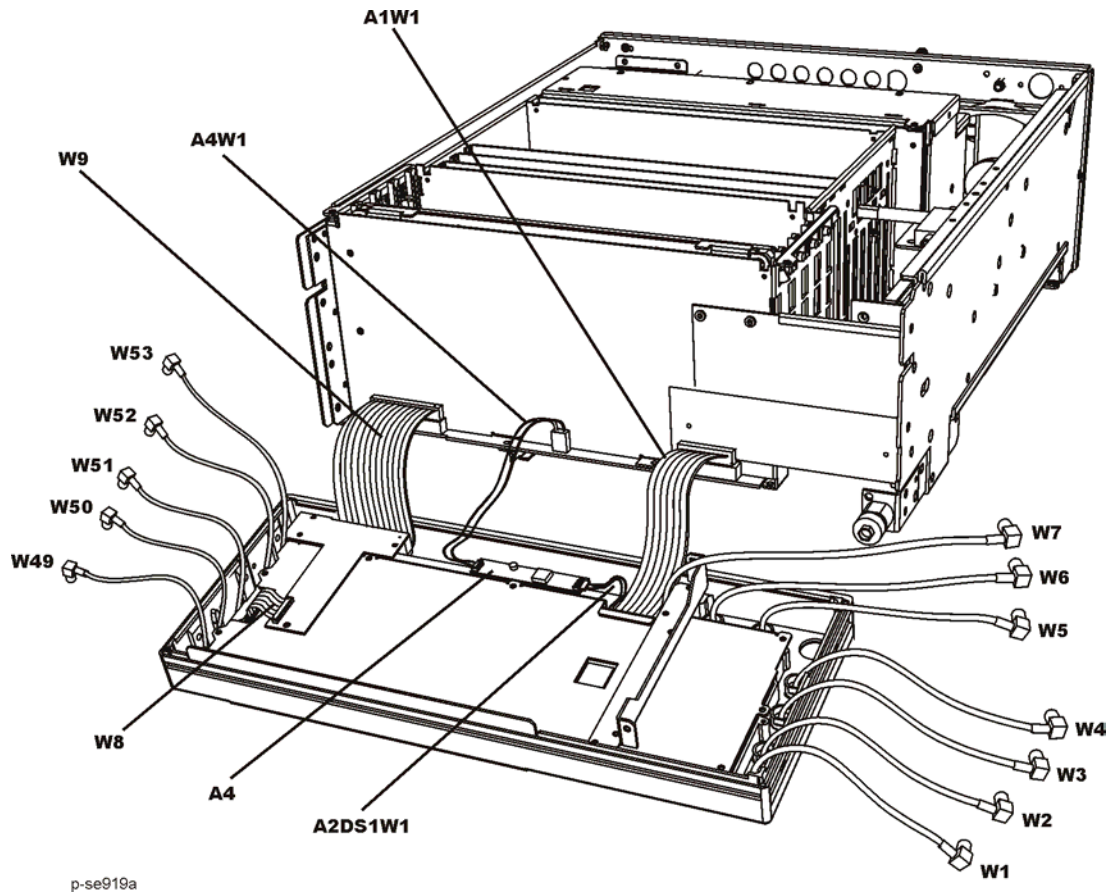
Figure 3-12 Inside Front Panel
