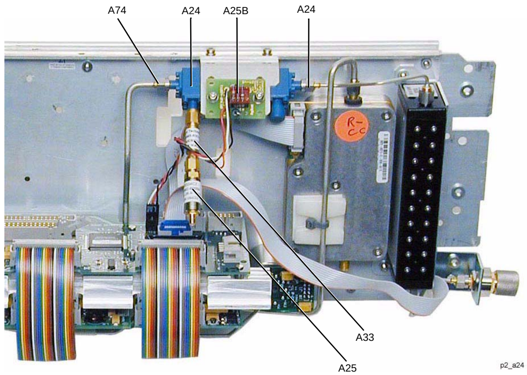
Figure 2-44 A33 6 dB PAD
