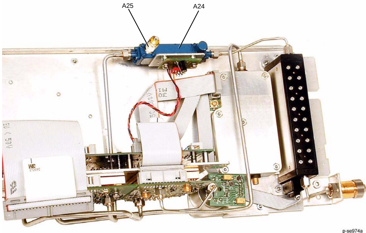
Figure 2-34 A25 40 GHz High Band Detector
