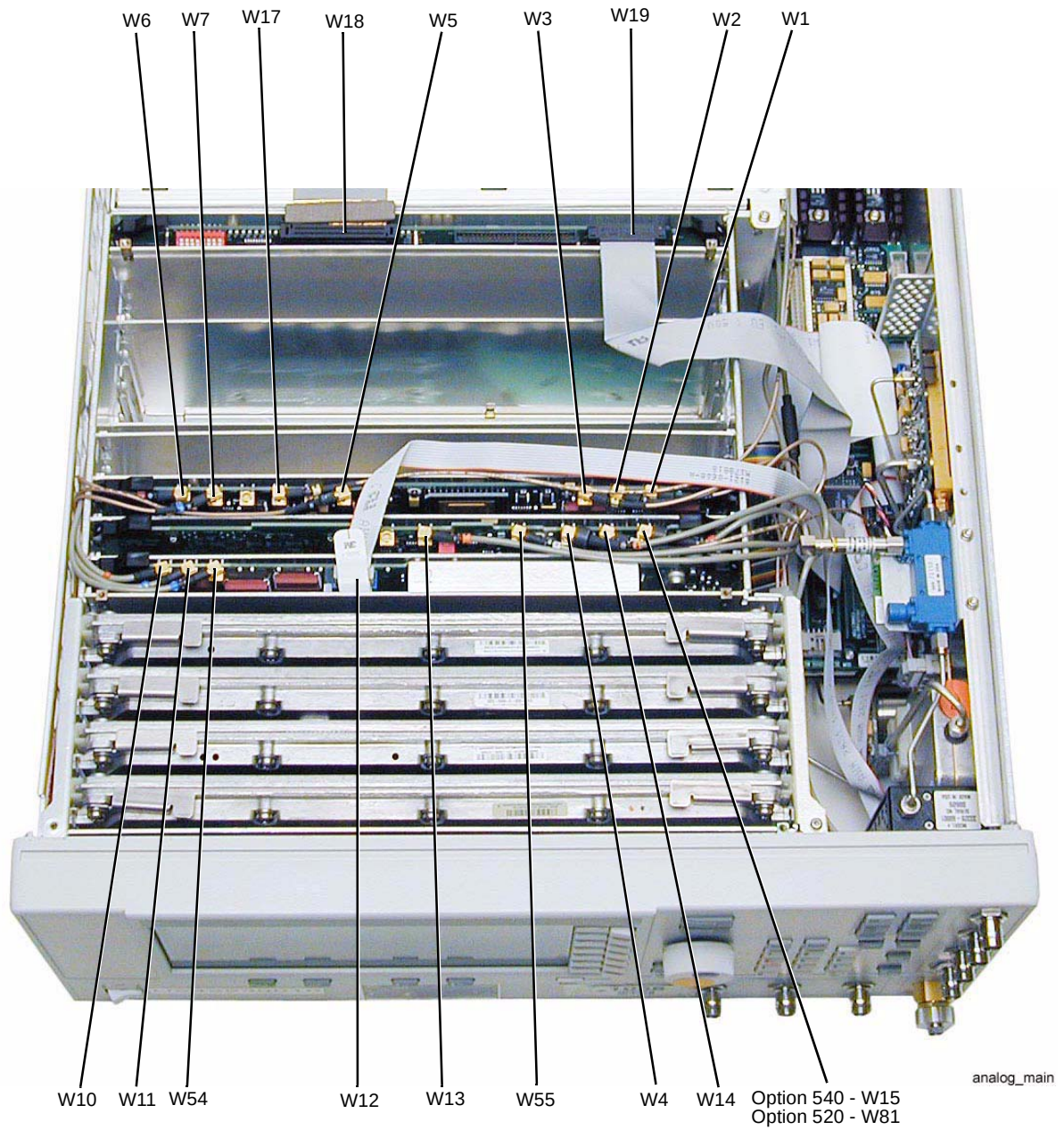
Figure 3-13 Top View (E8247C and E8257C)
