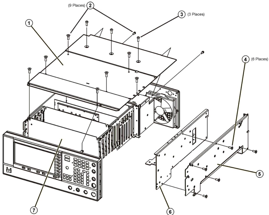
Figure 3-35 Main Chassis with Inside Cover and Right-Side Support Wall
